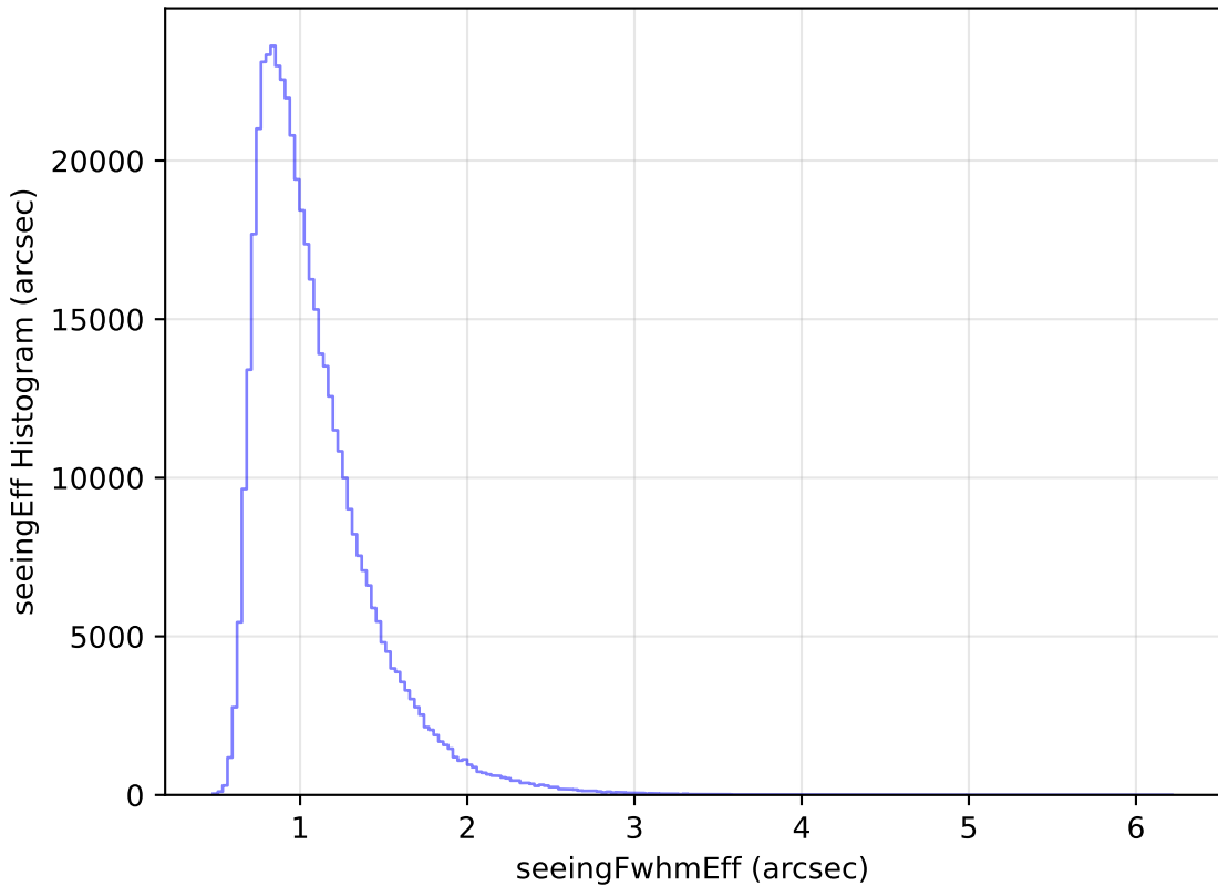
no_high_blob_v3.3_10yrs WFD i band: seeingEff Histogram
