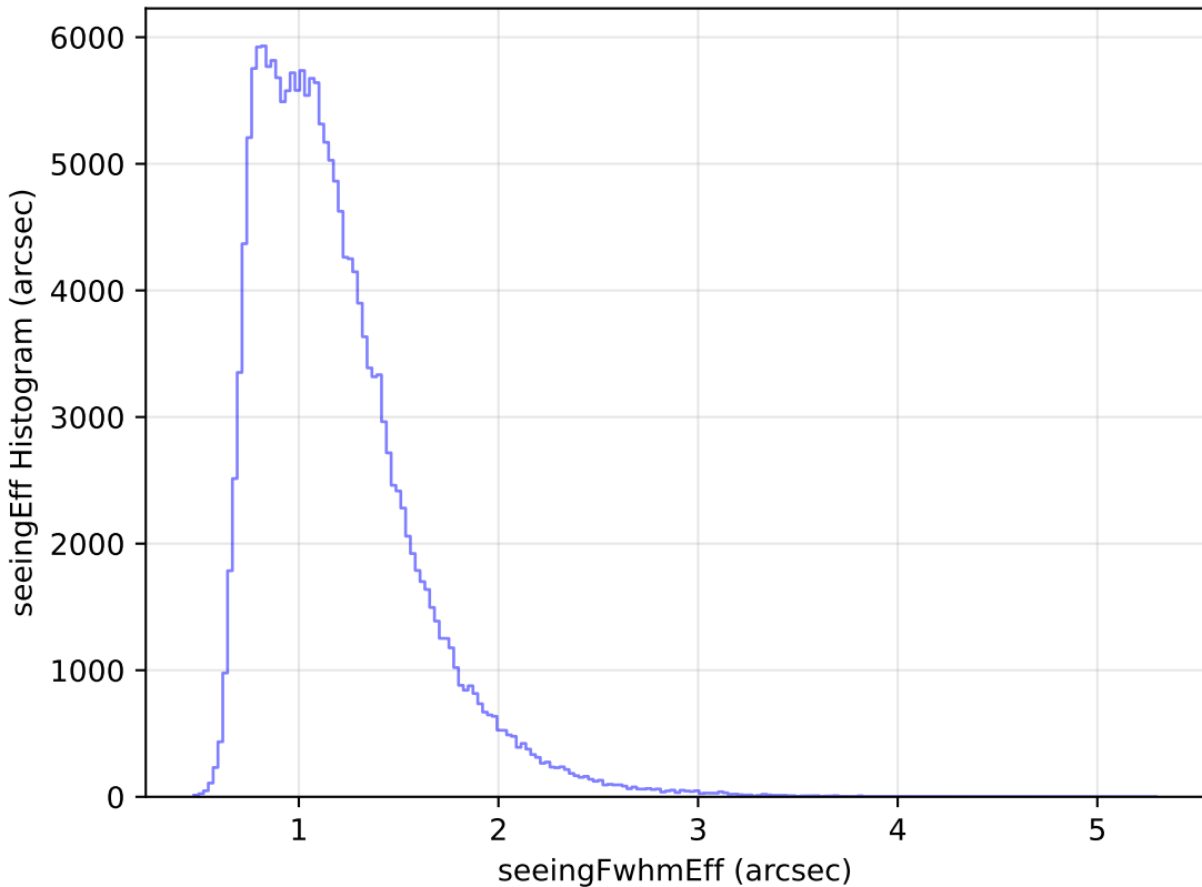
no_high_blob_v3.3_10yrs WFD g band: seeingEff Histogram
