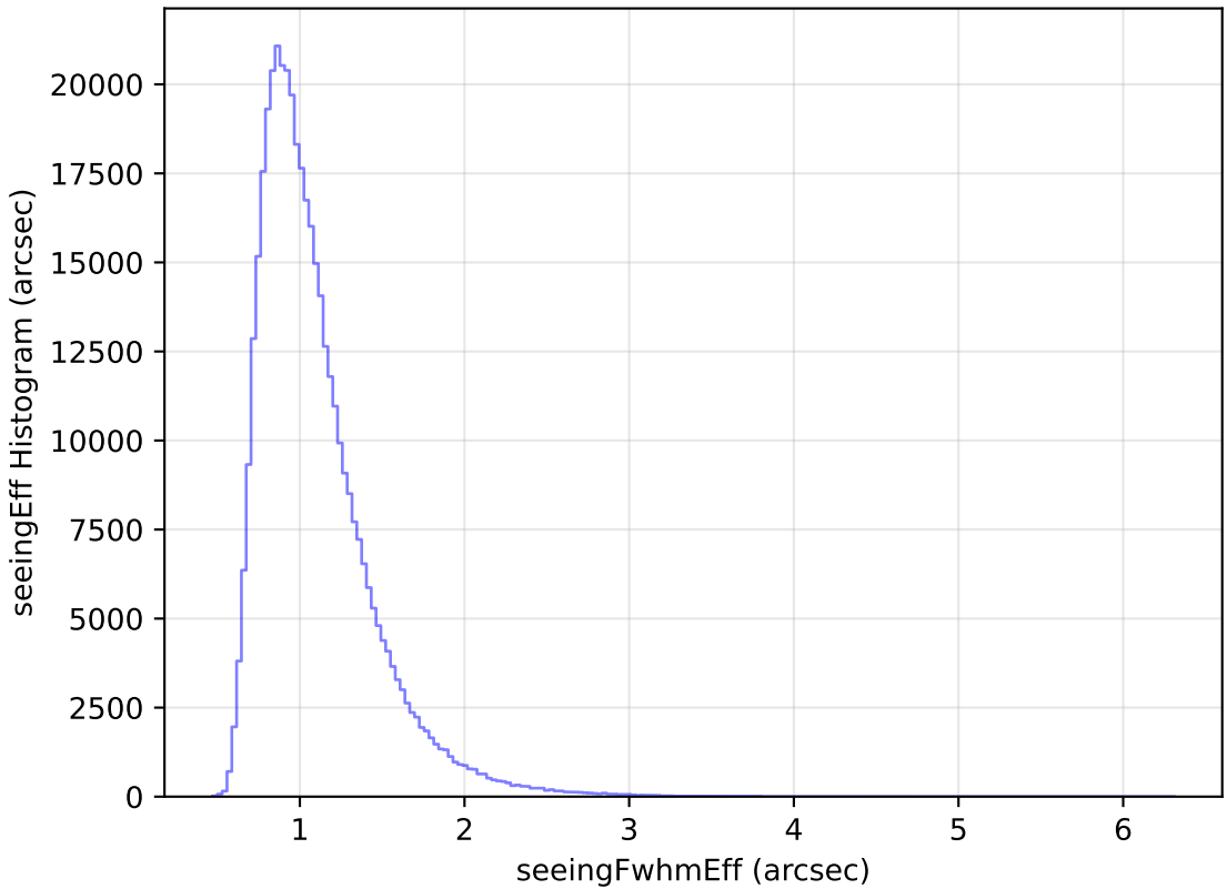
no_high_blob_v3.3_10yrs All sky z band: seeingEff Histogram
