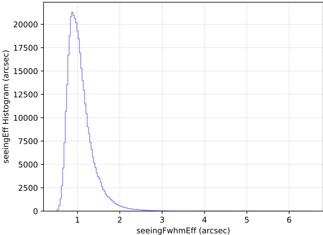
no_high_blob_v3.3_10yrs All sky y band: seeingEff Histogram
