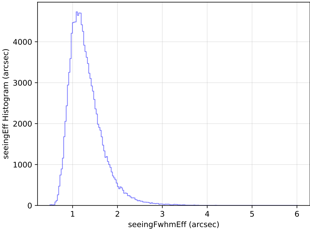
no_high_blob_v3.3_10yrs All sky u band: seeingEff Histogram
