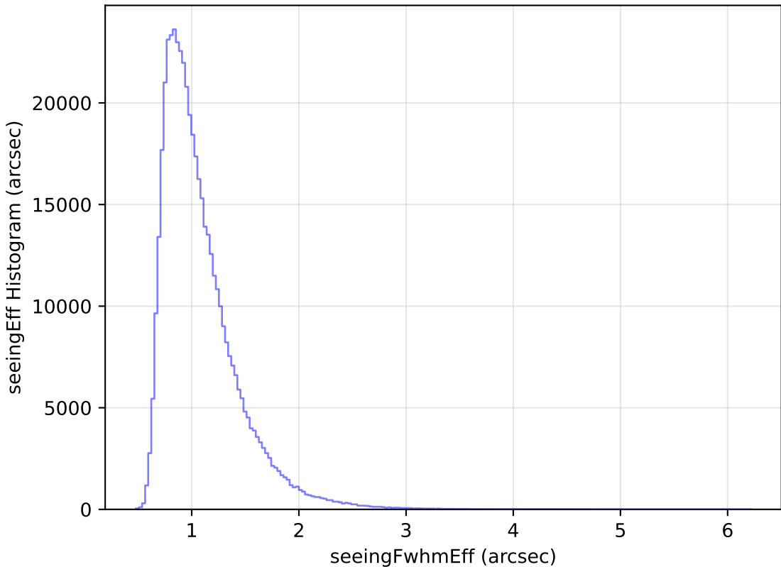
no_high_blob_v3.3_10yrs All sky i band: seeingEff Histogram
