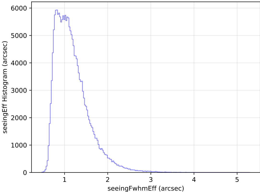
no_high_blob_v3.3_10yrs All sky g band: seeingEff Histogram
