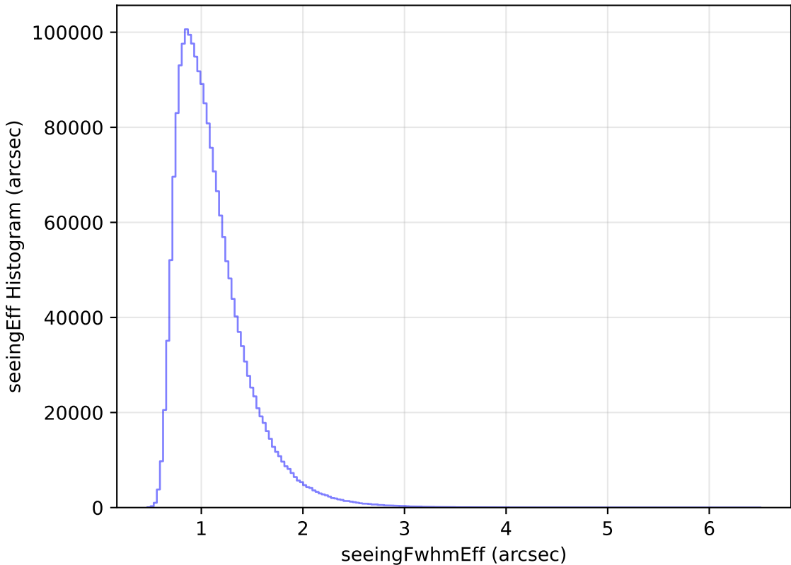
no_high_blob_v3.3_10yrs All sky all bands: seeingEff Histogram
