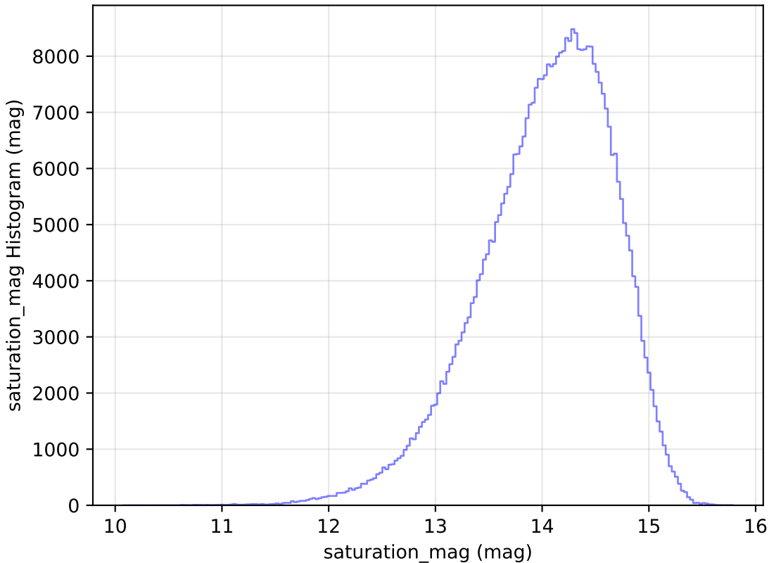
no_high_blob_v3.3_10yrs WFD z band: saturation_mag Histogram
