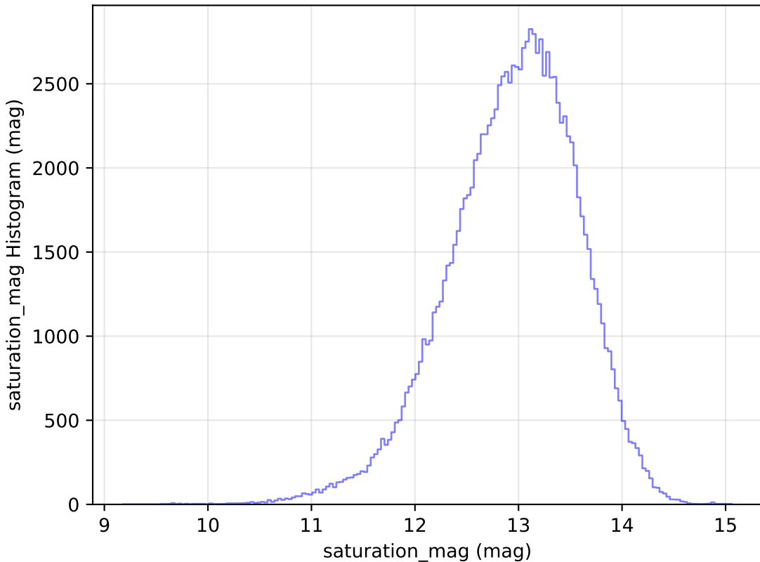
no_high_blob_v3.3_10yrs WFD u band: saturation_mag Histogram
