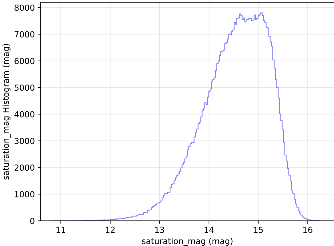
no_high_blob_v3.3_10yrs WFD r band: saturation_mag Histogram
