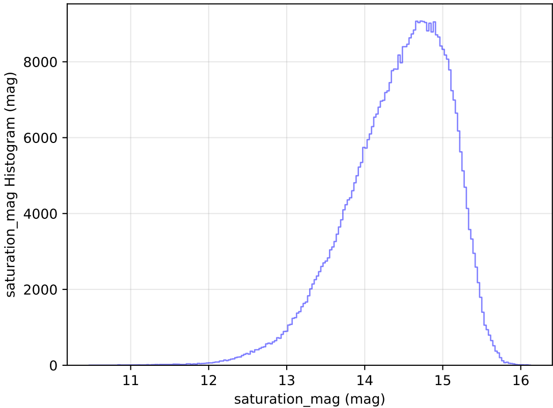
no_high_blob_v3.3_10yrs WFD i band: saturation_mag Histogram
