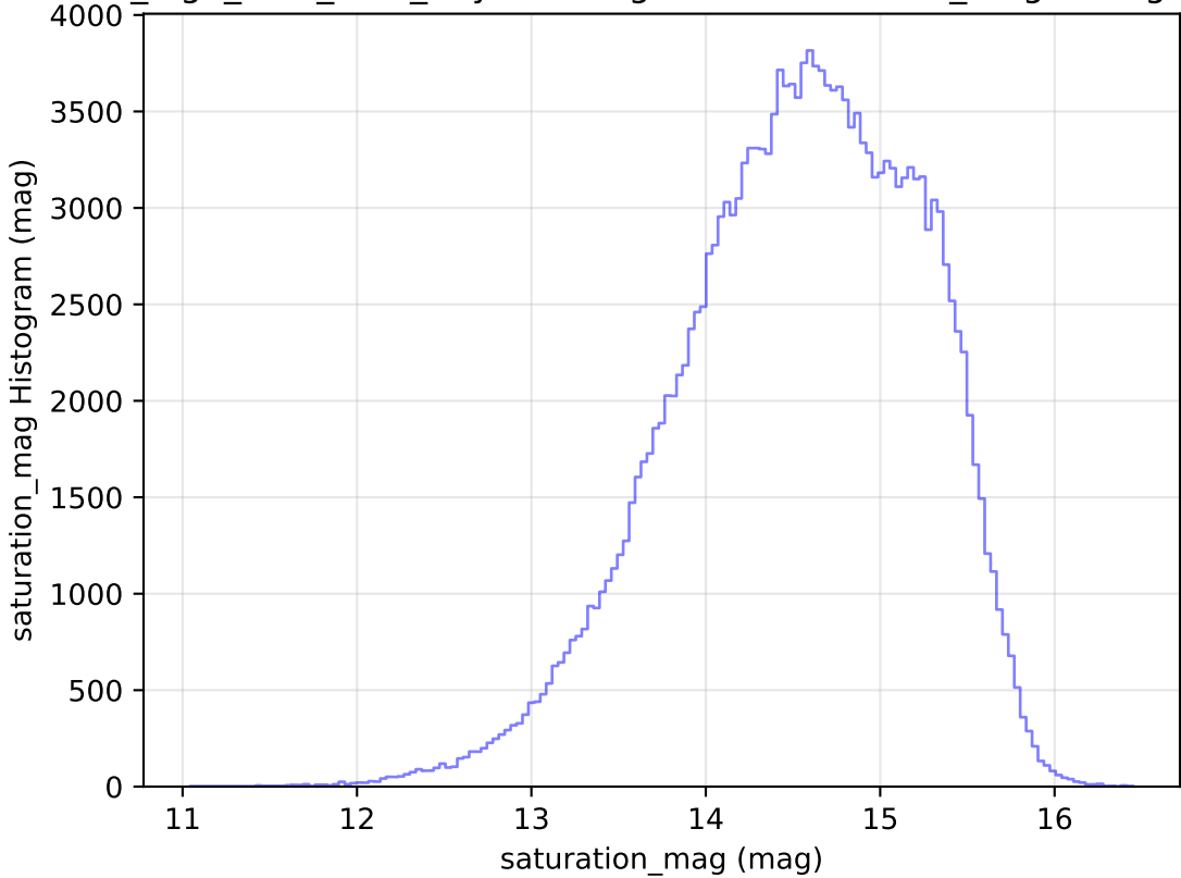
no_high_blob_v3.3_10yrs WFD g band: saturation_mag Histogram
