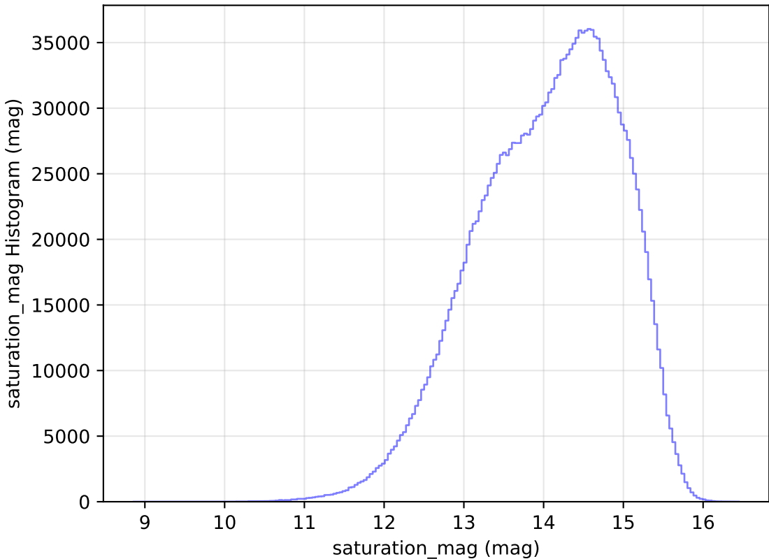
no_high_blob_v3.3_10yrs WFD all bands: saturation_mag Histogram
