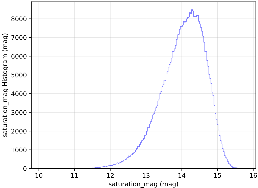
no_high_blob_v3.3_10yrs All sky z band: saturation_mag Histogram
