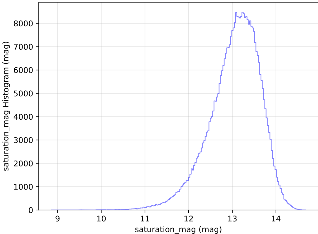
no_high_blob_v3.3_10yrs All sky y band: saturation_mag Histogram
