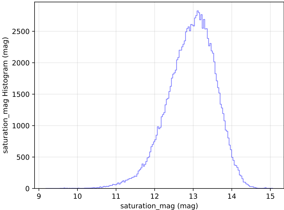
no_high_blob_v3.3_10yrs All sky u band: saturation_mag Histogram
