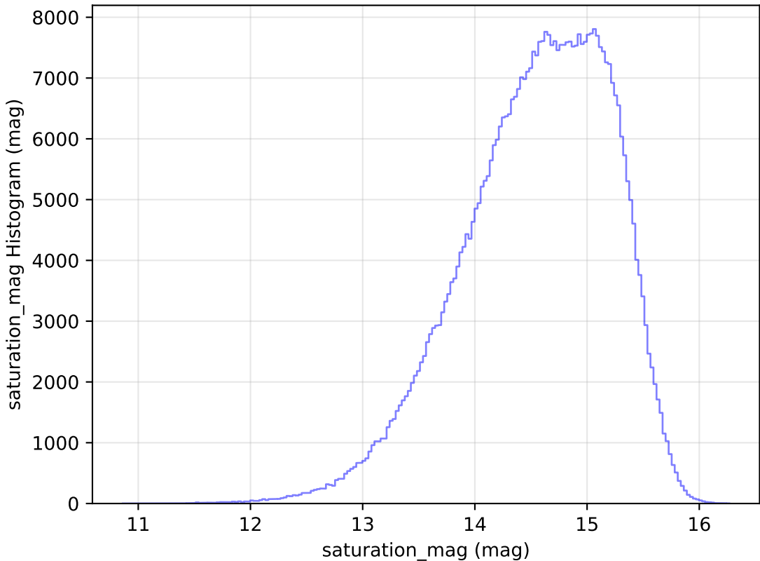
no_high_blob_v3.3_10yrs All sky r band: saturation_mag Histogram
