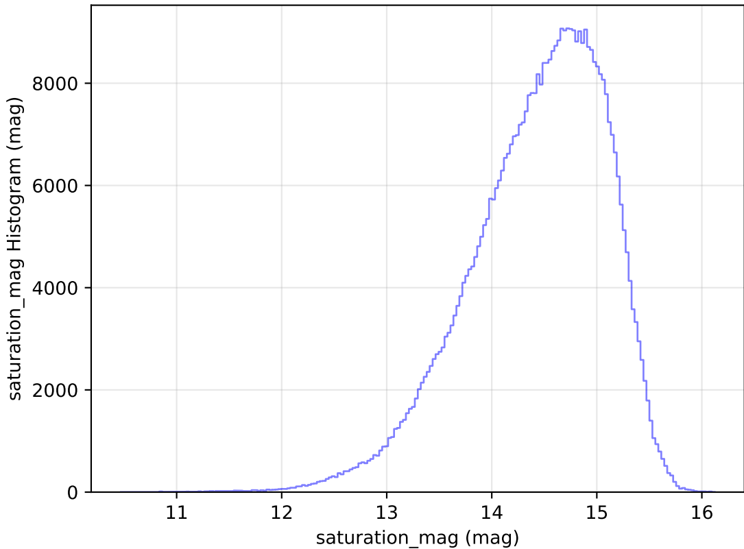
no_high_blob_v3.3_10yrs All sky i band: saturation_mag Histogram
