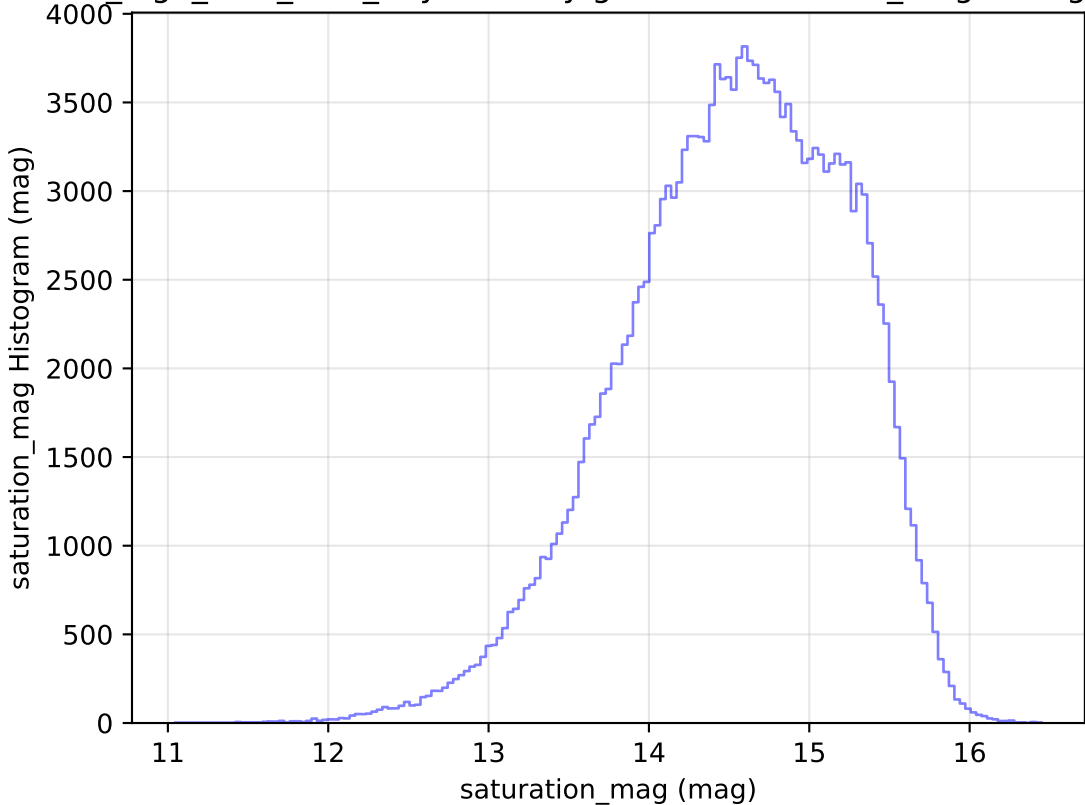
no_high_blob_v3.3_10yrs All sky g band: saturation_mag Histogram
