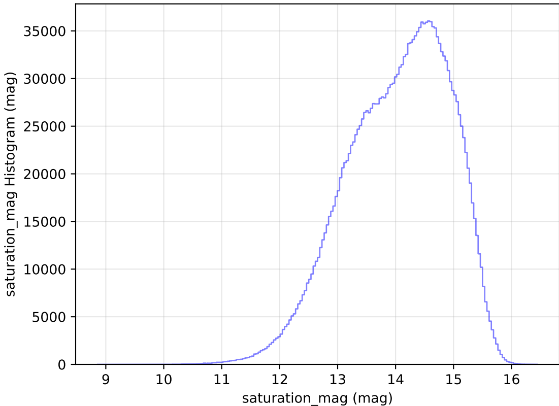
no_high_blob_v3.3_10yrs All sky all bands: saturation_mag Histogram
