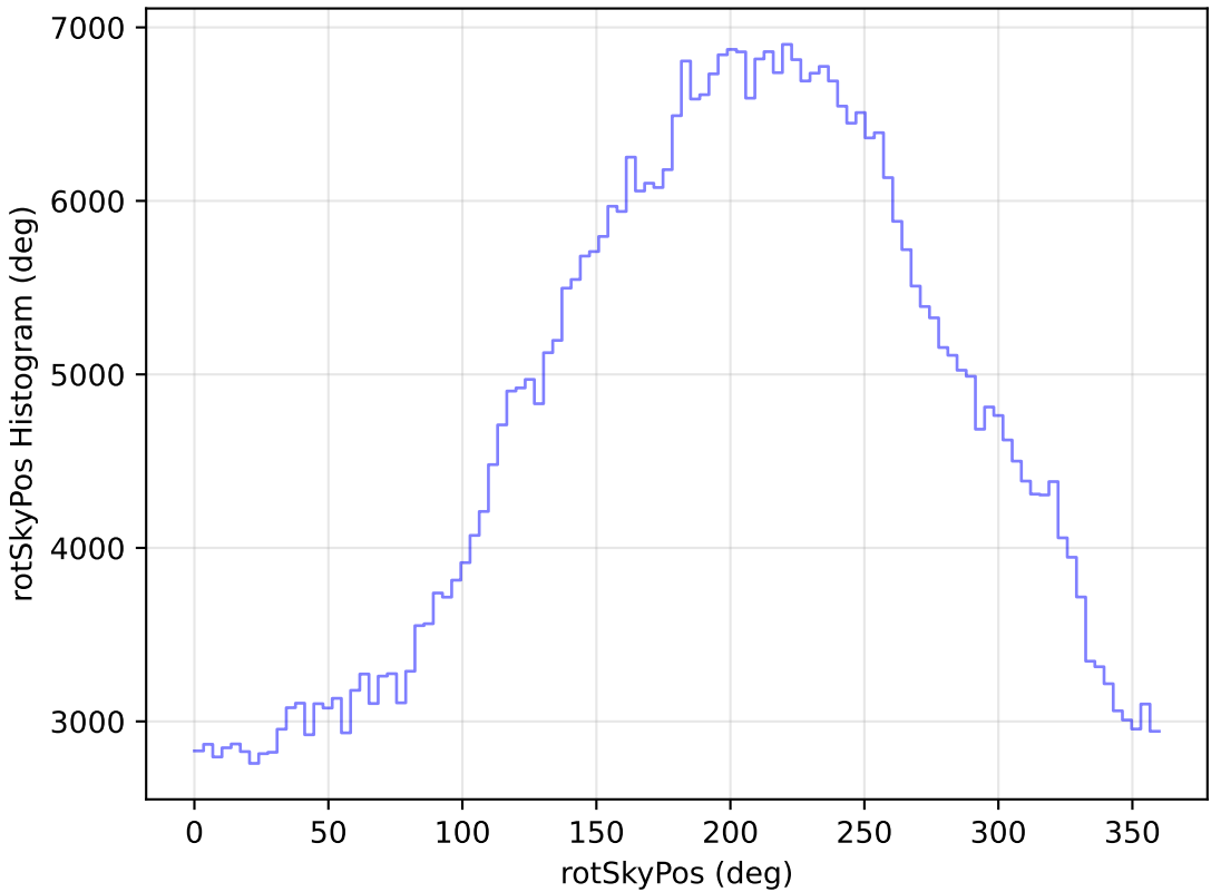
no_high_blob_v3.3_10yrs WFD i band: rotSkyPos Histogram
