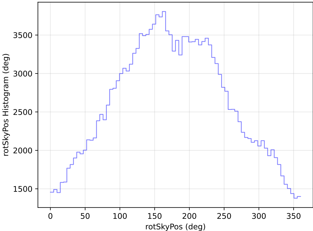
no_high_blob_v3.3_10yrs WFD g band: rotSkyPos Histogram
