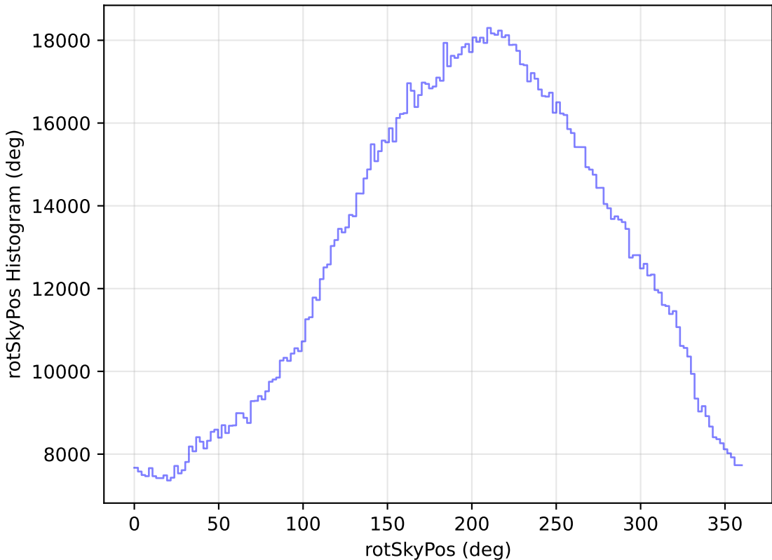
no_high_blob_v3.3_10yrs WFD all bands: rotSkyPos Histogram
