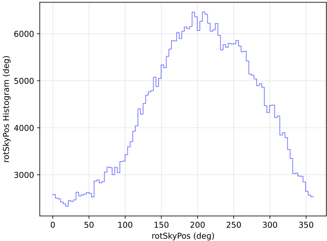
no_high_blob_v3.3_10yrs All sky z band: rotSkyPos Histogram
