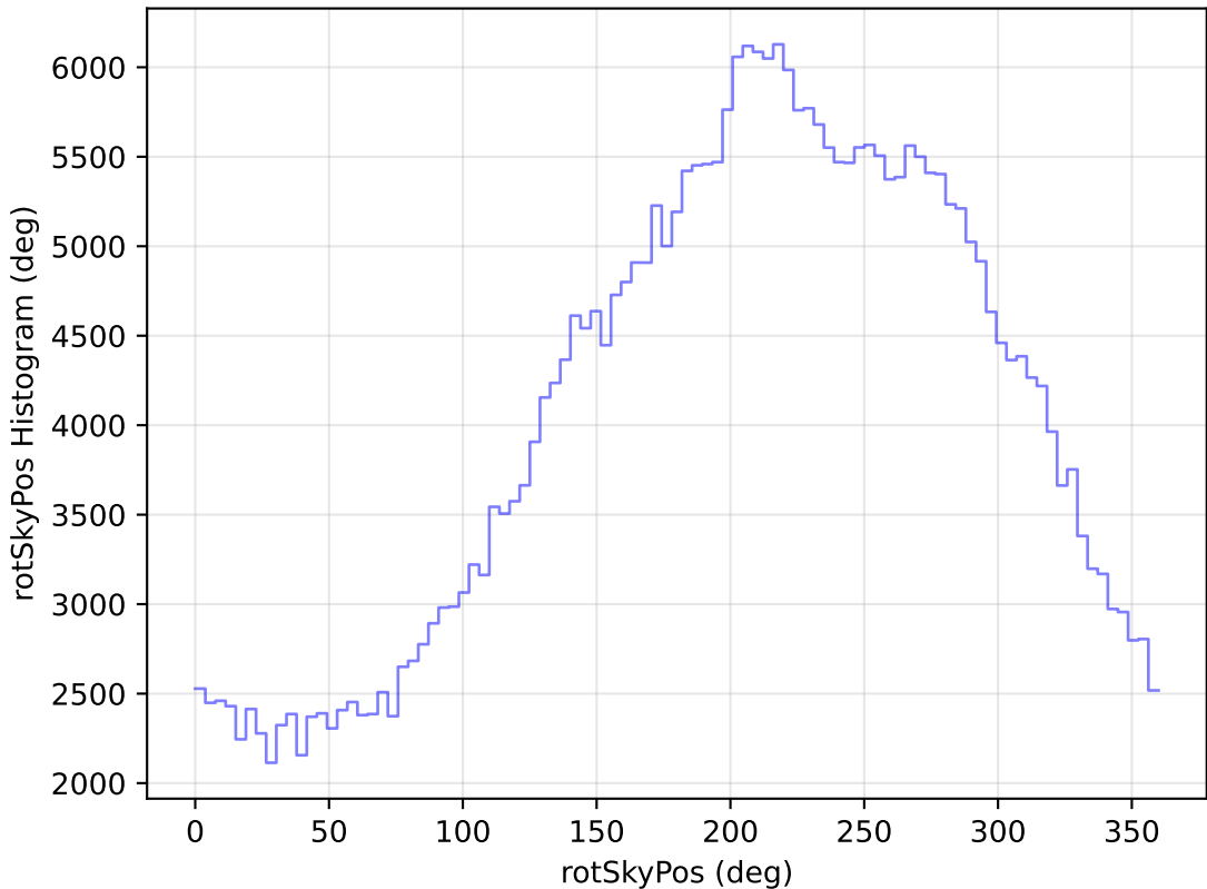
no_high_blob_v3.3_10yrs All sky y band: rotSkyPos Histogram
