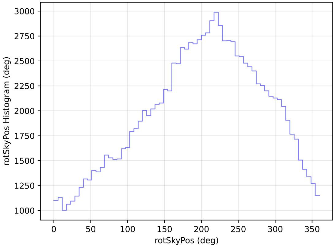
no_high_blob_v3.3_10yrs All sky u band: rotSkyPos Histogram
