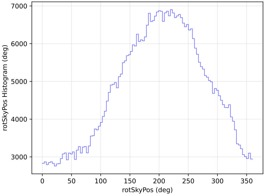
no_high_blob_v3.3_10yrs All sky i band: rotSkyPos Histogram
