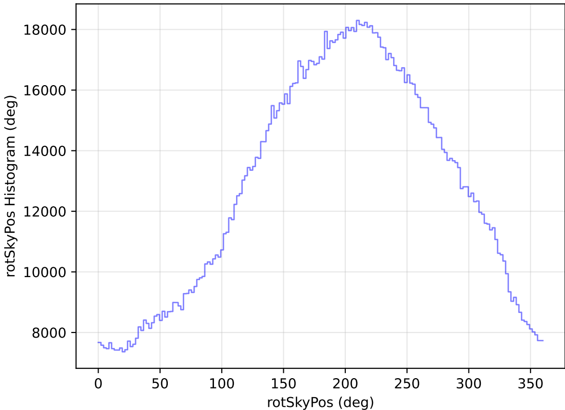
no_high_blob_v3.3_10yrs All sky all bands: rotSkyPos Histogram
