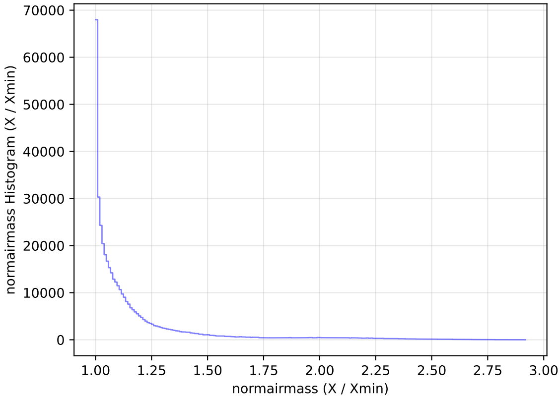
no_high_blob_v3.3_10yrs WFD z band: normairmass Histogram
