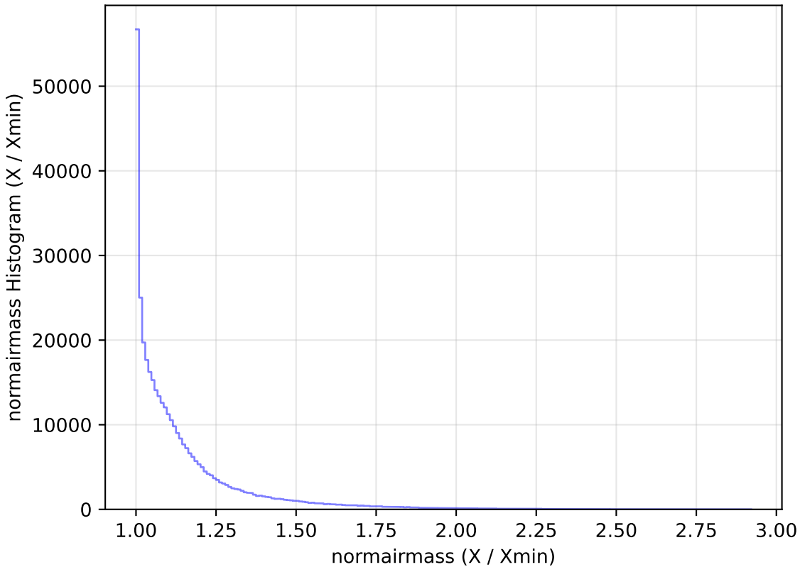
no_high_blob_v3.3_10yrs WFD y band: normairmass Histogram
