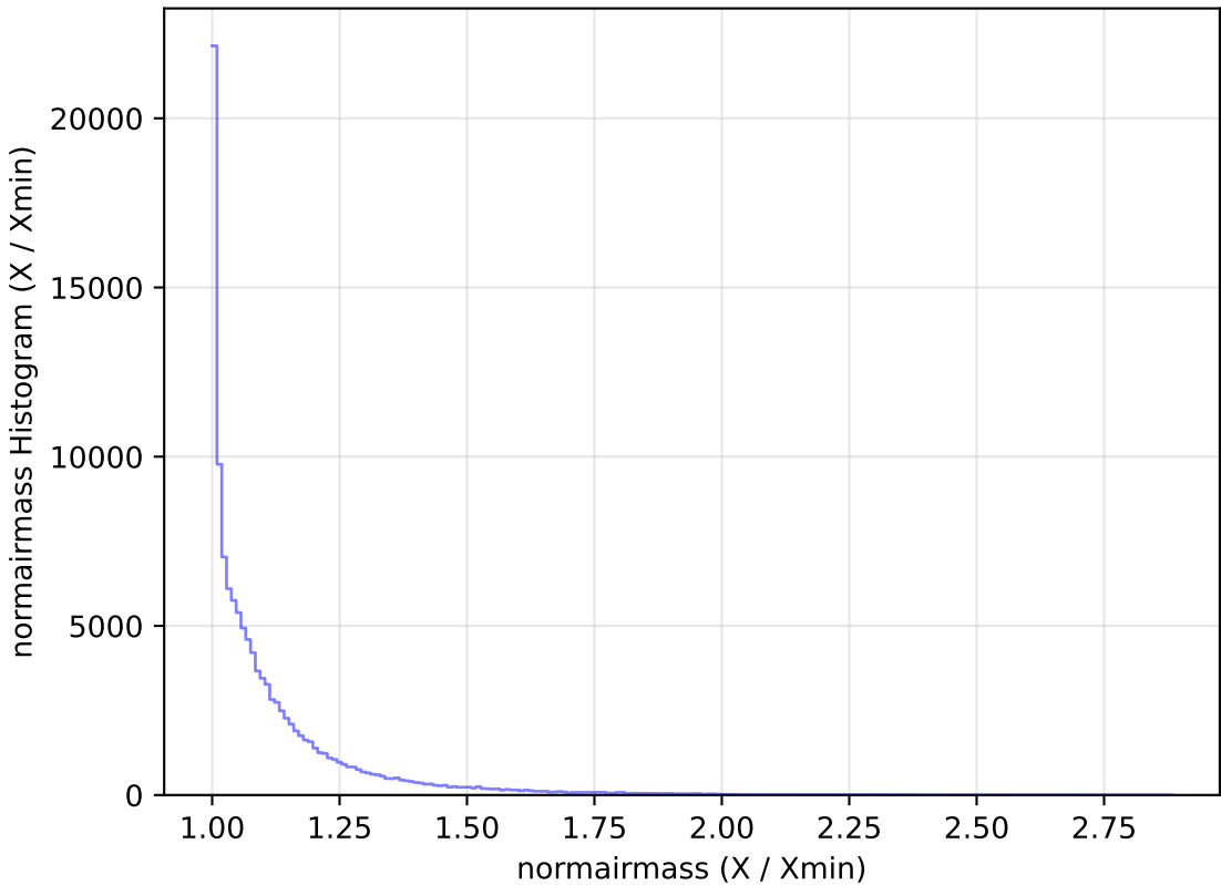
no_high_blob_v3.3_10yrs WFD u band: normairmass Histogram
