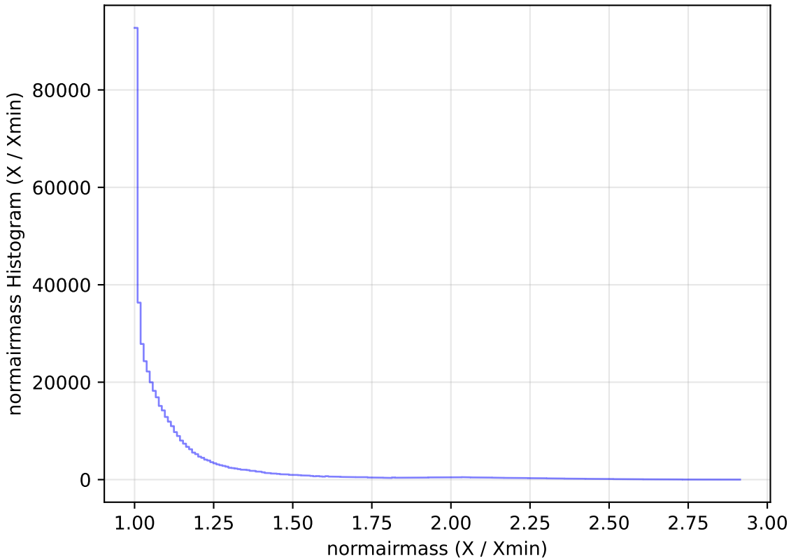
no_high_blob_v3.3_10yrs WFD i band: normairmass Histogram
