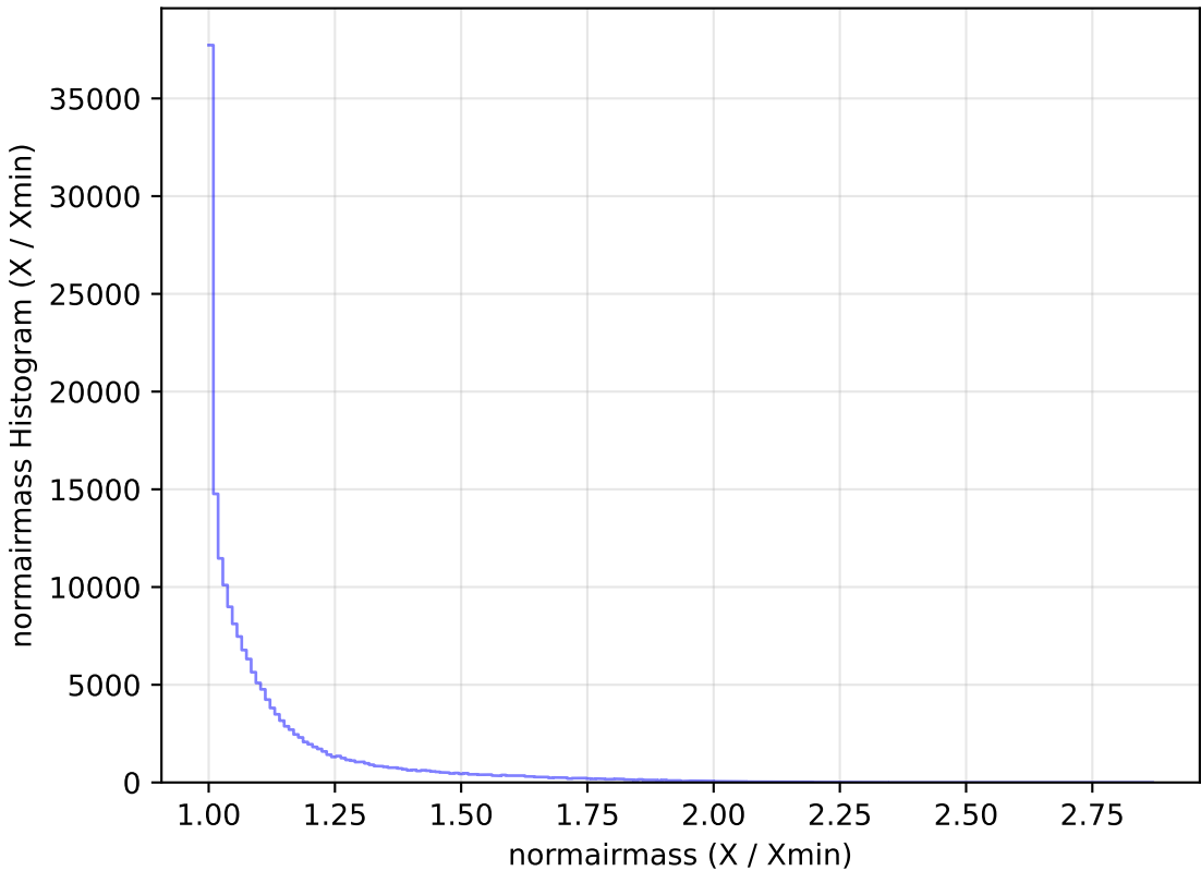
no_high_blob_v3.3_10yrs WFD g band: normairmass Histogram
