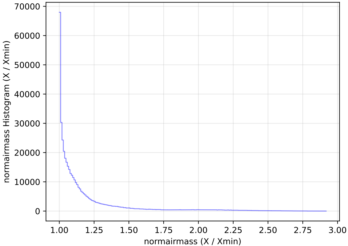
no_high_blob_v3.3_10yrs All sky z band: normairmass Histogram
