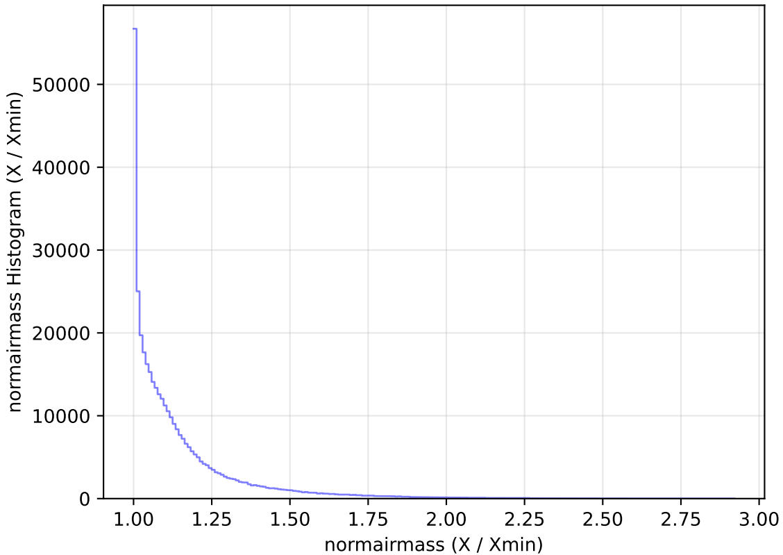
no_high_blob_v3.3_10yrs All sky y band: normairmass Histogram
