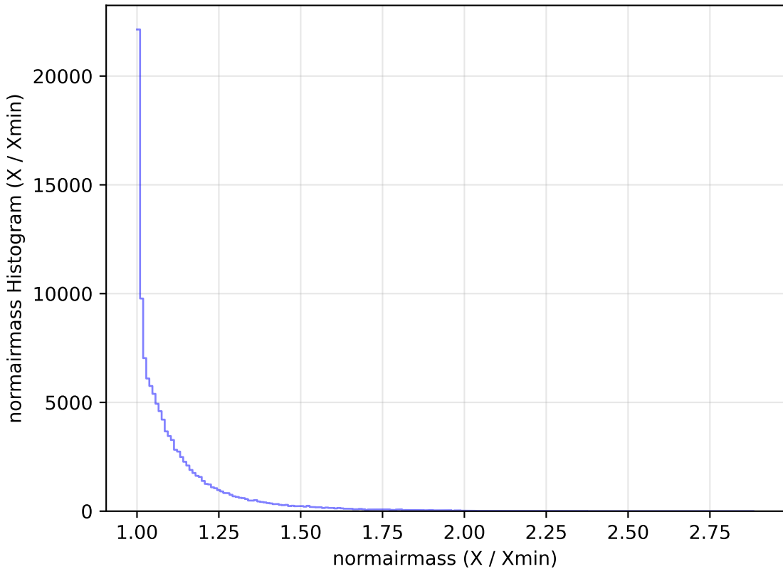
no_high_blob_v3.3_10yrs All sky u band: normairmass Histogram
