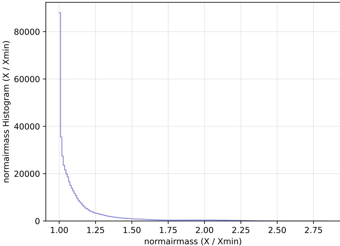
no_high_blob_v3.3_10yrs All sky r band: normairmass Histogram
