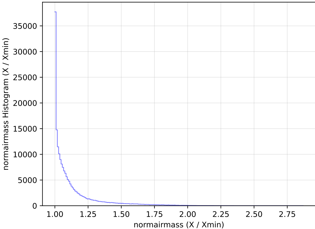
no_high_blob_v3.3_10yrs All sky g band: normairmass Histogram
