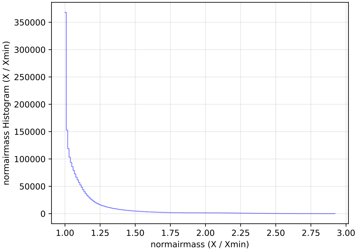
no_high_blob_v3.3_10yrs All sky all bands: normairmass Histogram
