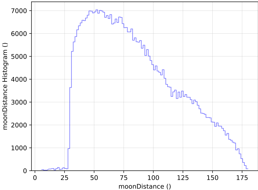
no_high_blob_v3.3_10yrs WFD z band: moonDistance Histogram
