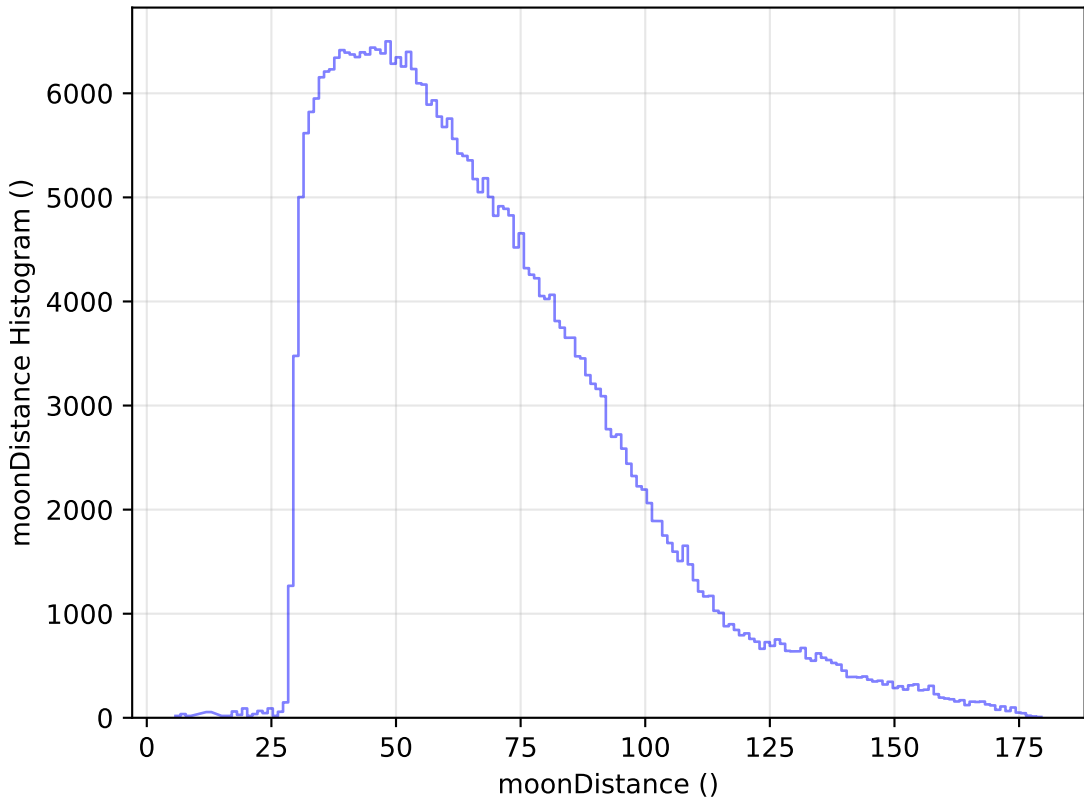
no_high_blob_v3.3_10yrs WFD y band: moonDistance Histogram
