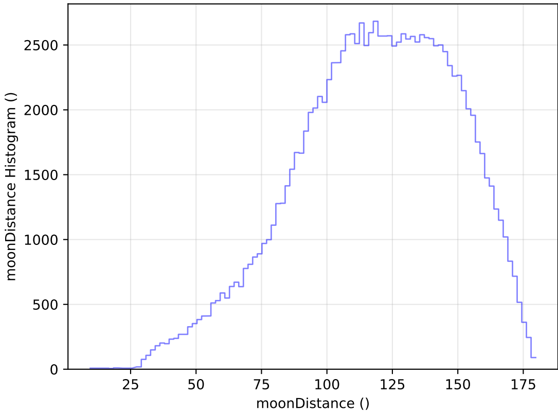
no_high_blob_v3.3_10yrs WFD u band: moonDistance Histogram
