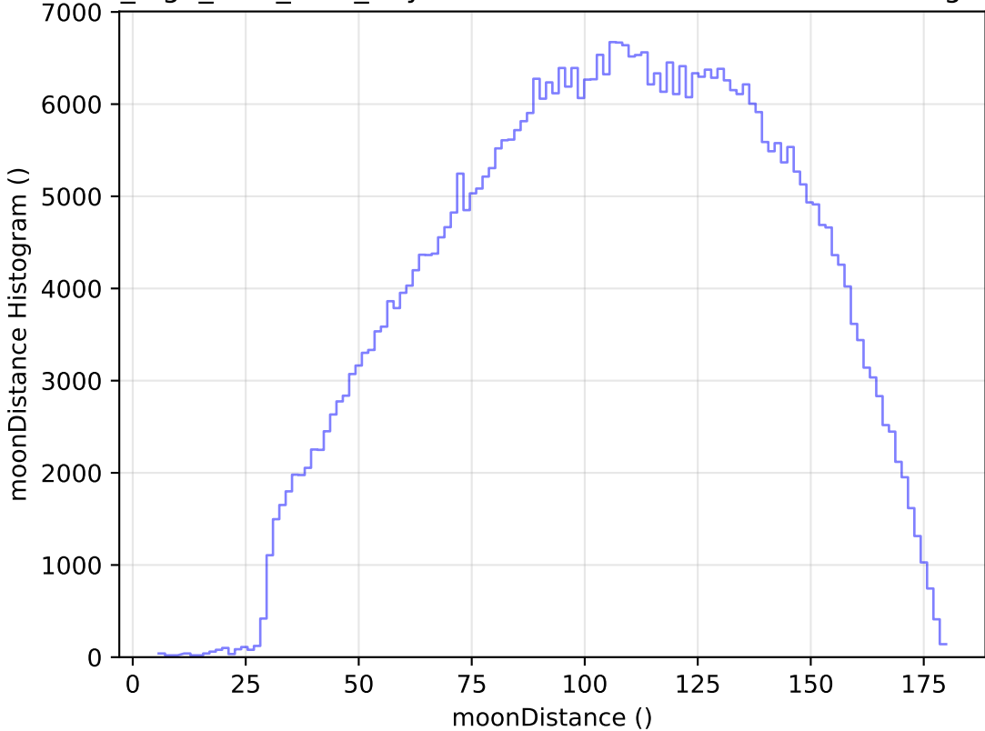
no_high_blob_v3.3_10yrs WFD r band: moonDistance Histogram
