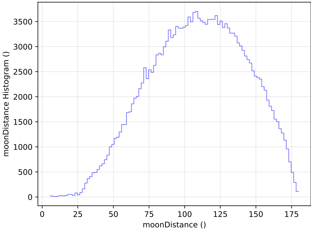
no_high_blob_v3.3_10yrs WFD g band: moonDistance Histogram
