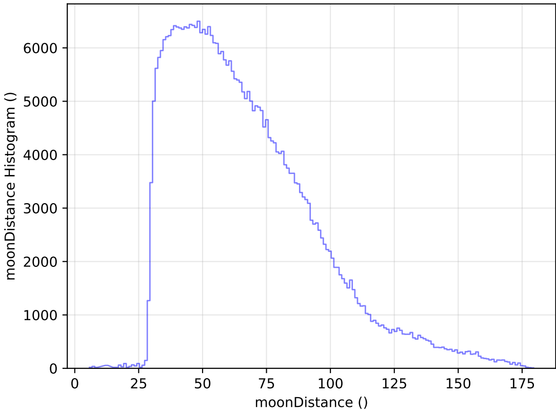
no_high_blob_v3.3_10yrs All sky y band: moonDistance Histogram
