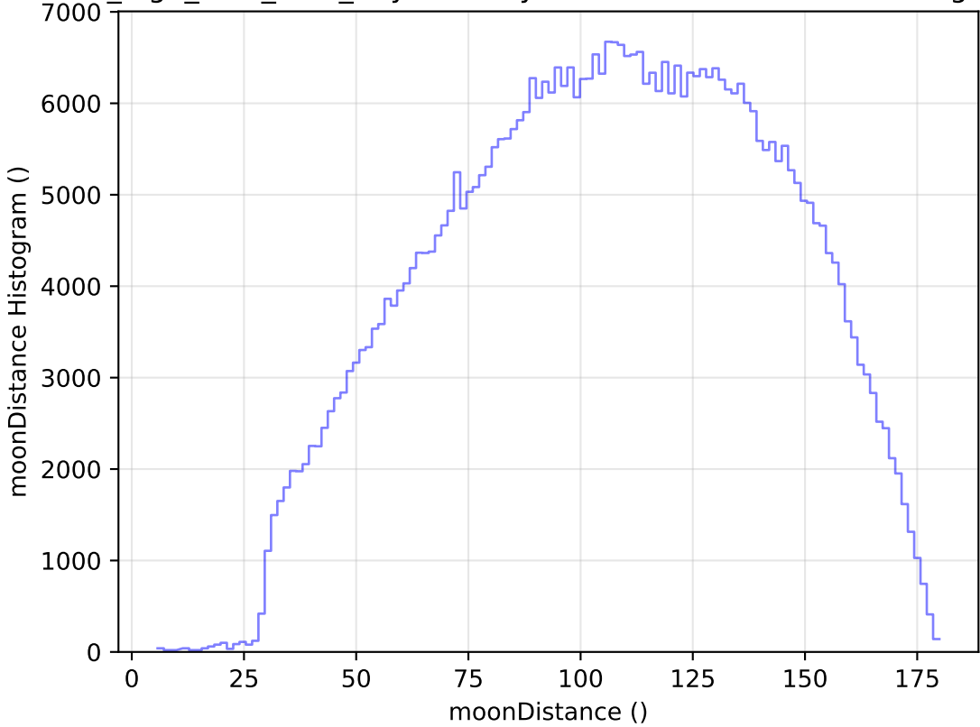
no_high_blob_v3.3_10yrs All sky r band: moonDistance Histogram
