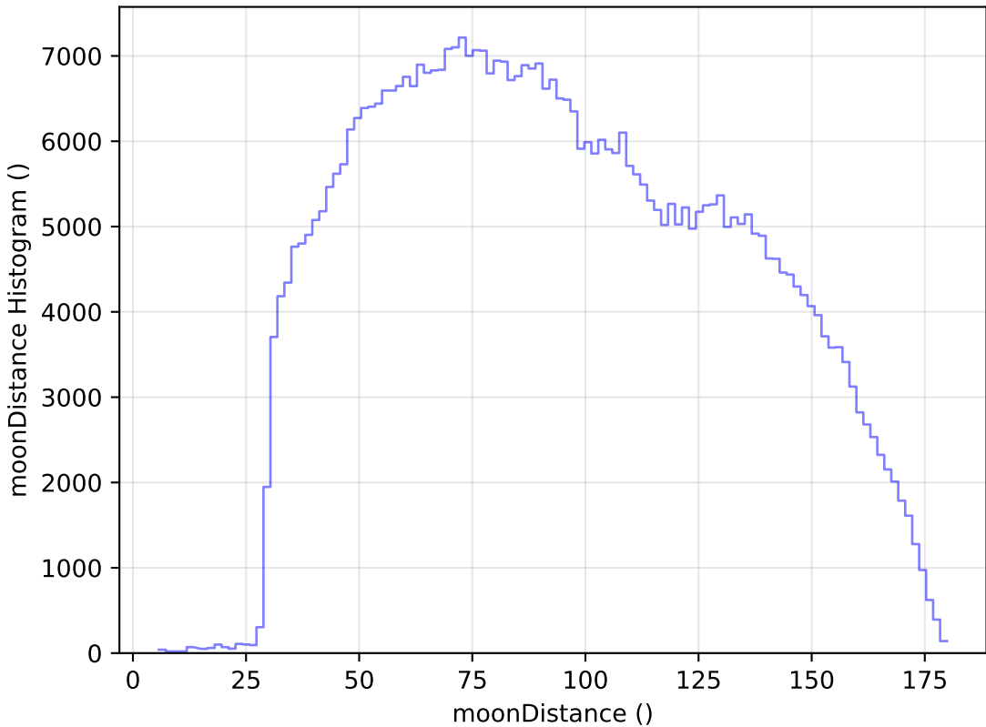
no_high_blob_v3.3_10yrs All sky i band: moonDistance Histogram
