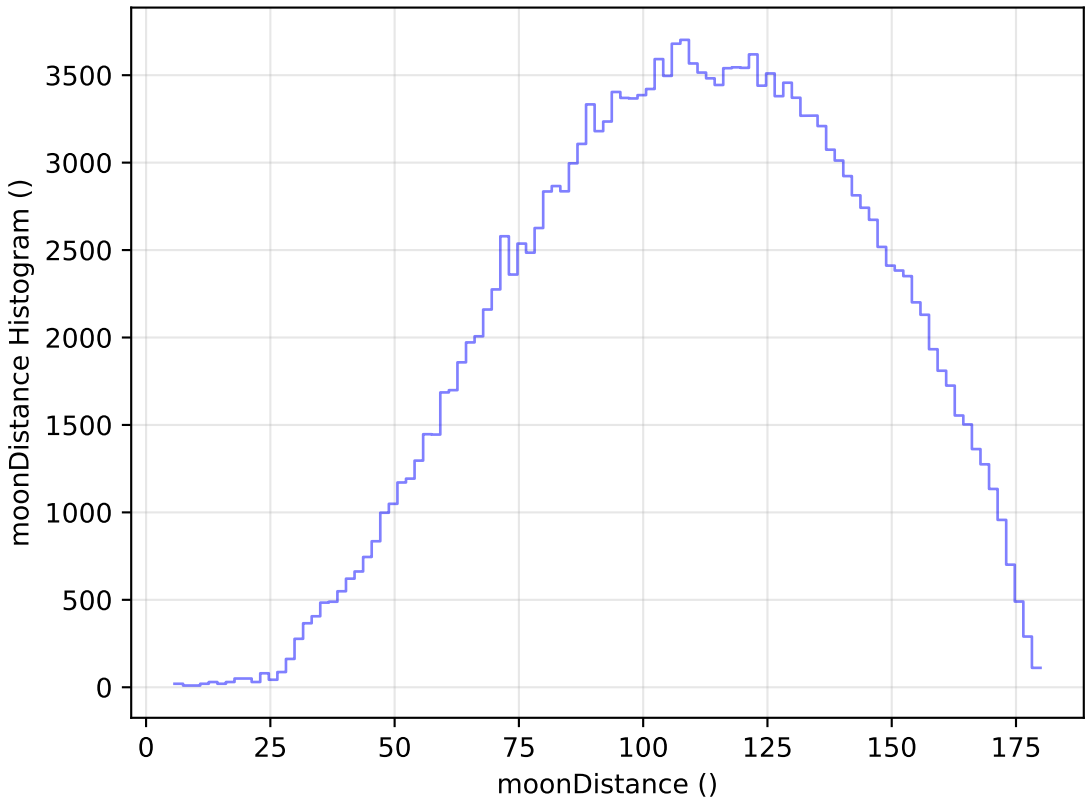
no_high_blob_v3.3_10yrs All sky g band: moonDistance Histogram
