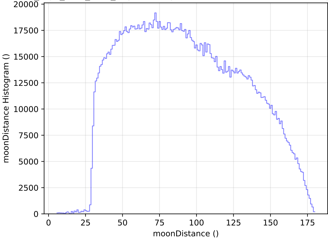
no_high_blob_v3.3_10yrs All sky all bands: moonDistance Histogram
